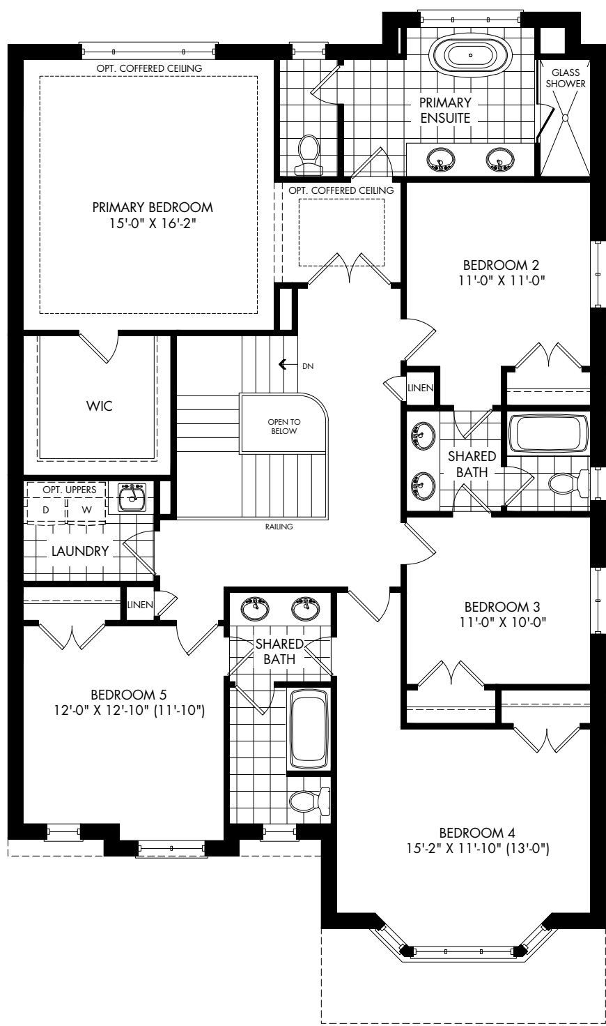
OPTIONAL SECOND FLOOR ELEV. A 5 BEDROOM
