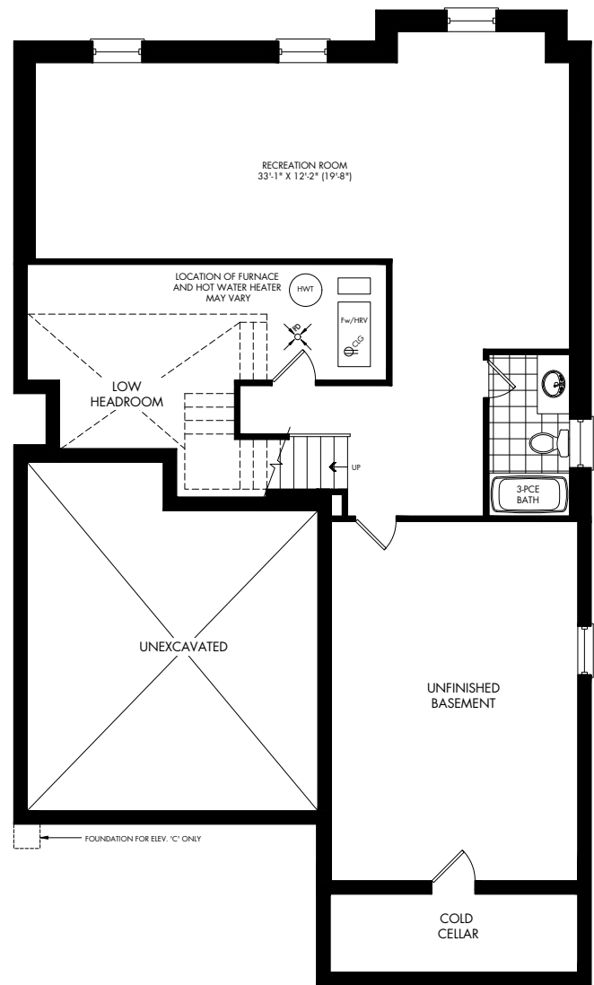
FINISHED BASEMENT ELEV. A, B & C
